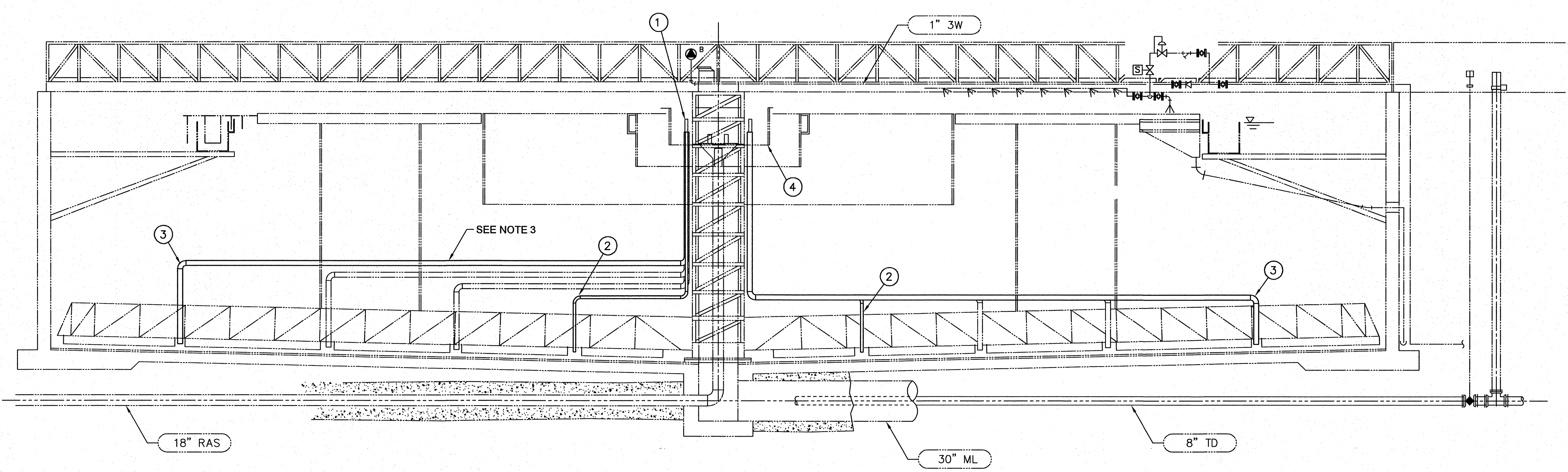
SECONDARY CLARIFIER 4 TYPICAL SECTION NO SCALE
