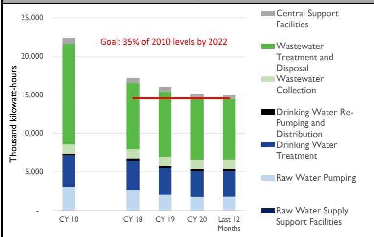
Electricity Use
