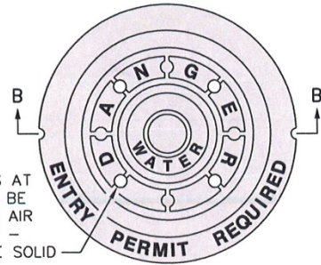
COVER FACE
