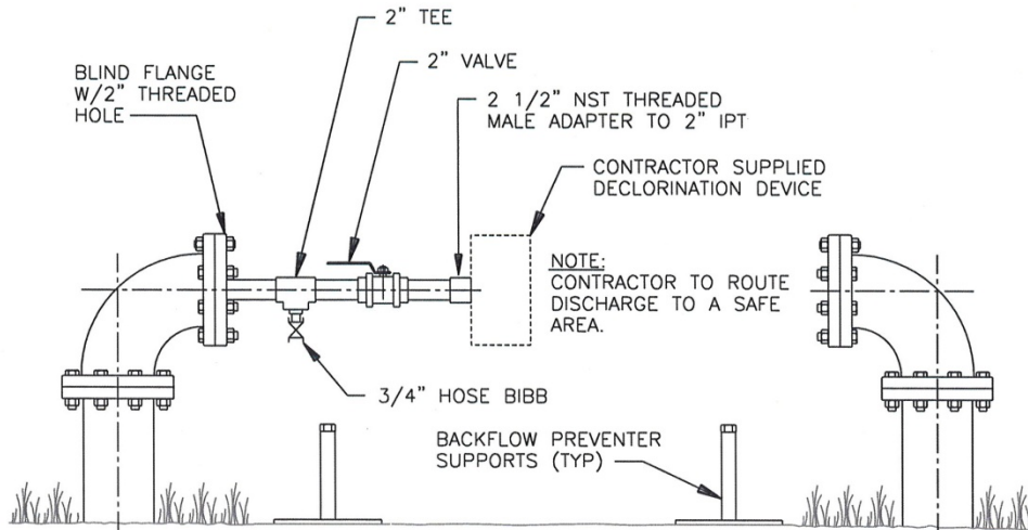
2" SAMPLING CONNECTION ON BACKFLOW PREVENTER TYPICAL 4" THRU 8"
