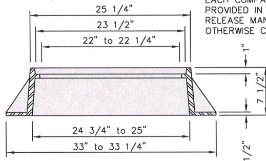
FRAME SECTION A-A
