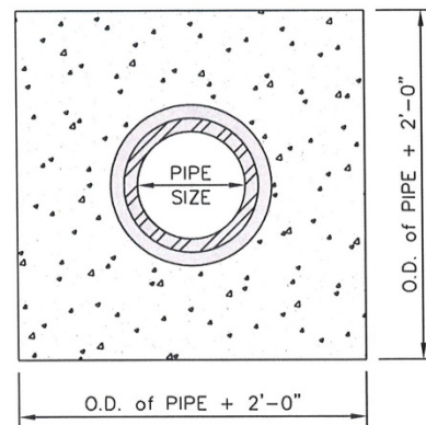
TRANSVERSE SECTION
