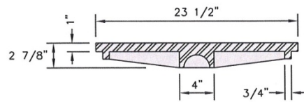
COVER SECTION B-B
