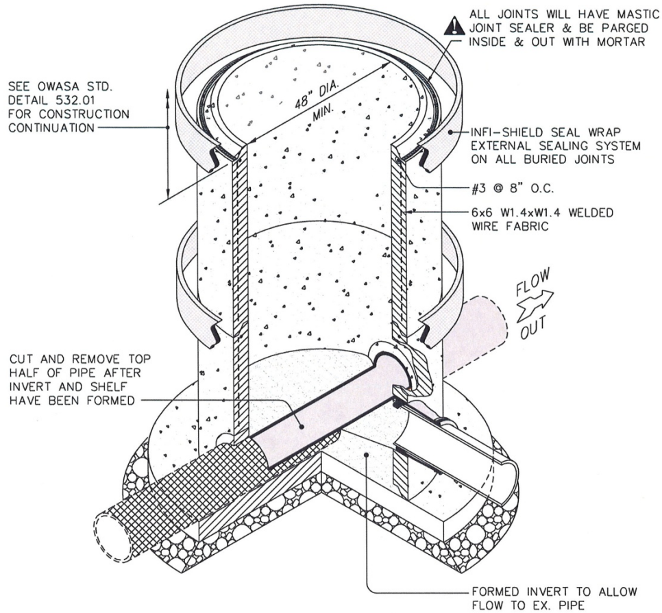
INVERT SECTION VIEW
