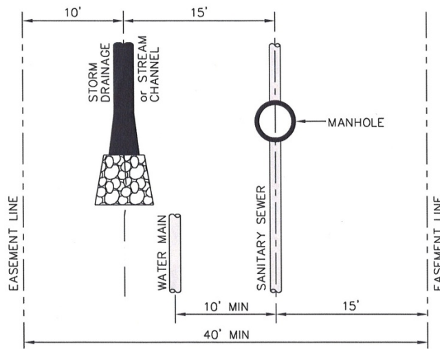
TYPICAL COMBINED EASEMENT
