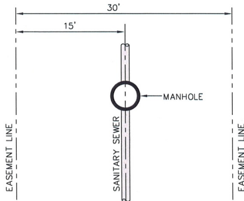
TYPICAL SEWER EASEMENT
